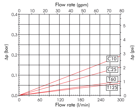
By-pass FA-2-10/11/20/21
