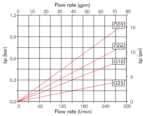
Element A-2-21
